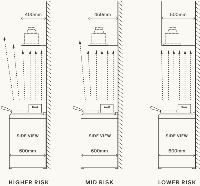
HEIGHT TOP OF COOKTOP TO BASE OF PRODUCT
